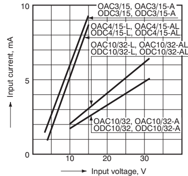
3. Input current vs. input voltage (OAC, ODC)
