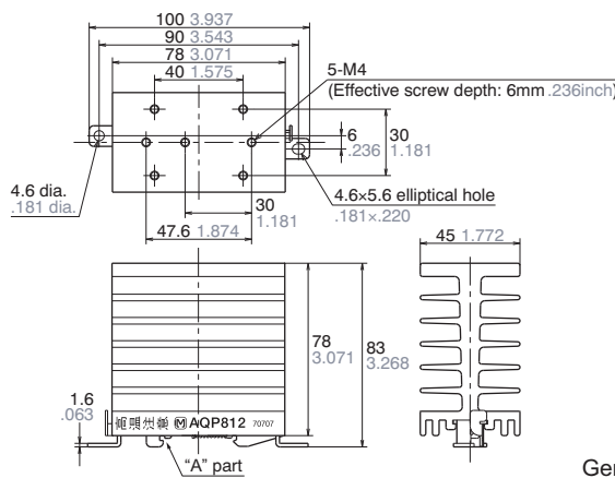
External dimensions
