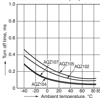
22-(1) Turn off time vs. ambient temperature characteristics (DC type)
