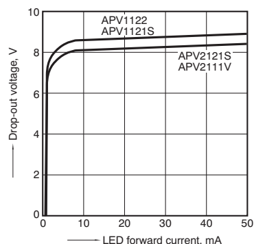
10. Drop-out voltage vs. LED forward current characteristics
