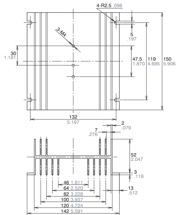
External dimensions
