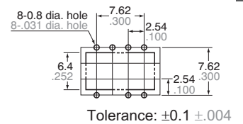
Recommended mounting pad (TOP VIEW)
