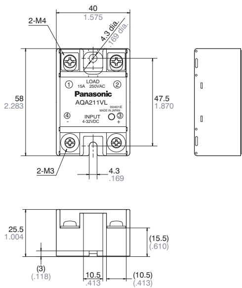
External dimensions
