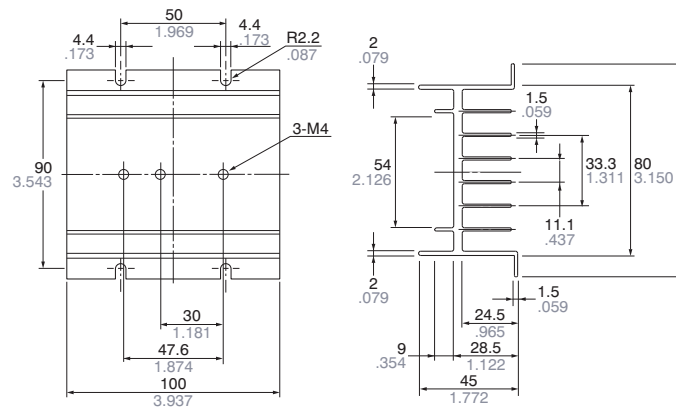
External dimensions
