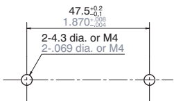
Mounting dimensions
