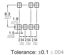
Recommended mounting pad (TOP VIEW)
