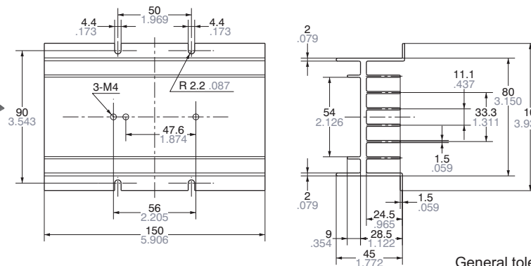
External dimensions
