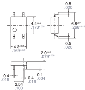
External dimensions
